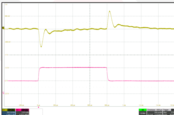
Figure 11: Output voltage response to step-change in load current 50%-100%-50% of Iout (max). No external load capacitance. Ch 1: Vout (500 mV/div). Ch 2: Iout (2 A/div). Timescale: 200μs/div.
