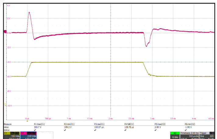
Figure 12: Output voltage response to step-change in input voltage (200 V - 300 V - 200 V) in 100 μS. Ch 2: Vout (2 V/div). Ch 1: Vin (100 V/div). Timescale: 500μs/div.
