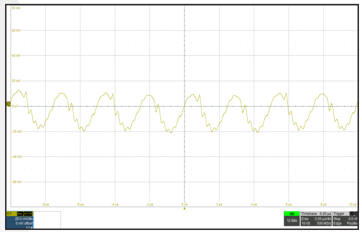
Figure 10: Output voltage ripple, Vout, at nominal input voltage and full rated load current (20 mV/div). Timescale: 2.00μs/div.
