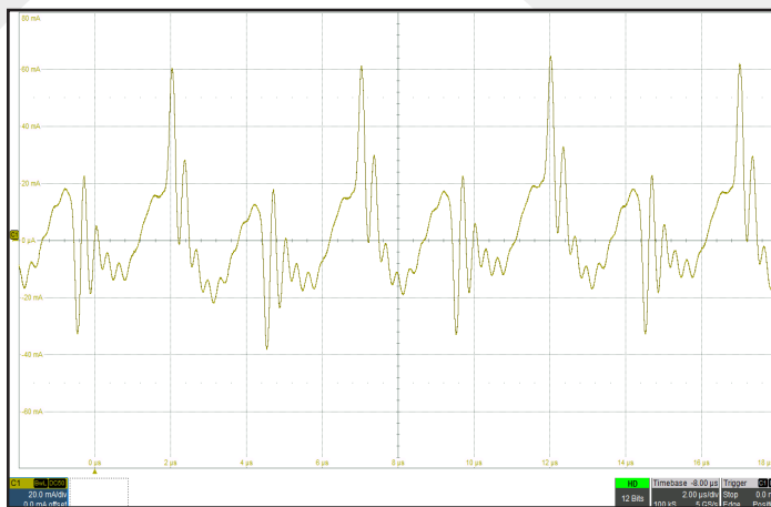
Figure 9: Input terminal current ripple, at full rated output current and nominal input voltage (20 mA/div). Timescale: 2.00μs/div. See Figure 17.
